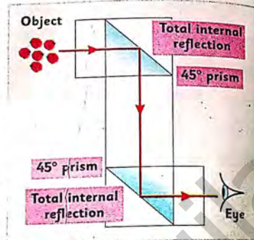
Fig. 9.8 A Periscope
