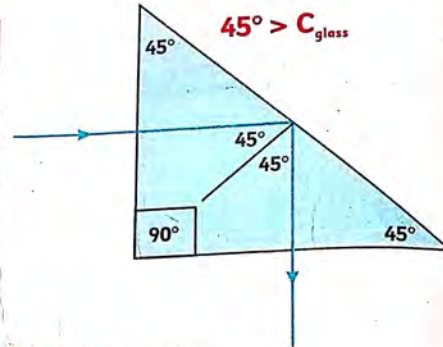
Fig. 9.7 Reflecting prism
