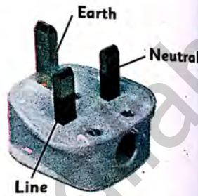
Fig. 11.15 Three pin plugs
