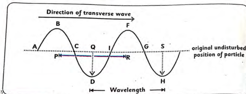
Fig. 10.6 Wave length
