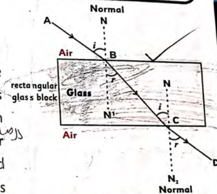
Fig. 9.1 Refraction of light
