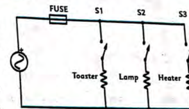
Fig. 11.12. House appliances in parallel
