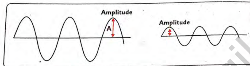
Fig. 10.7 Comparison of loud sound versus soft sound
