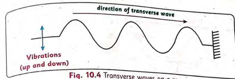
Fig. 10.4 Transverse waves on a rope
