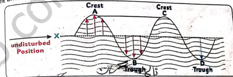
Fig. 10.5 Transverse wave
