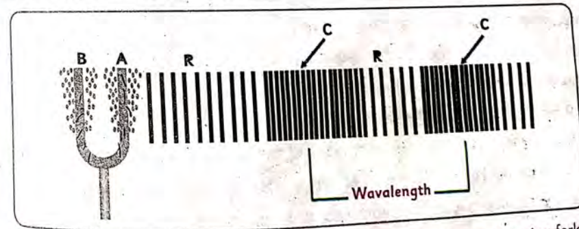
Fig. 10.2 Compressions and rarefactions of a longitudinal wave in tuning fork
