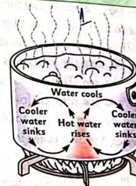
Fig 8.2: Convection currents
