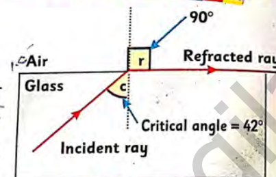
Fig 9.5 Critical angle
