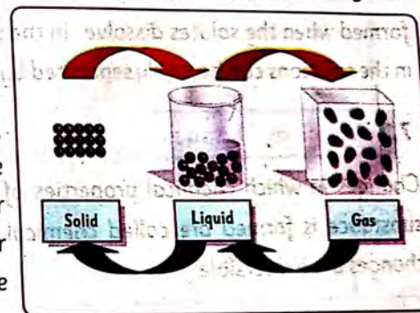
Fig. 7.1 Reversible Changes
