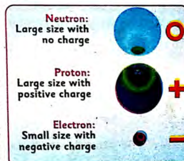
Fig. 6.1 Fundamental particles
