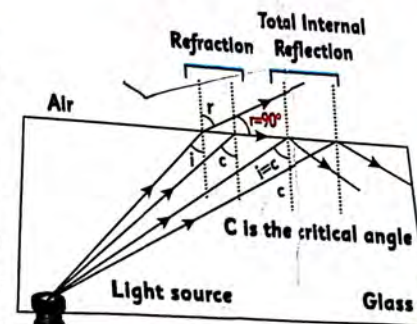
Fig. 9.6 Total Internal Reflection
