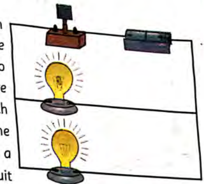
Fig. 11.3 Parallel circuit
