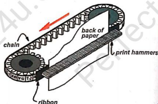
Figure 1.38 Chain Printer mechanism
