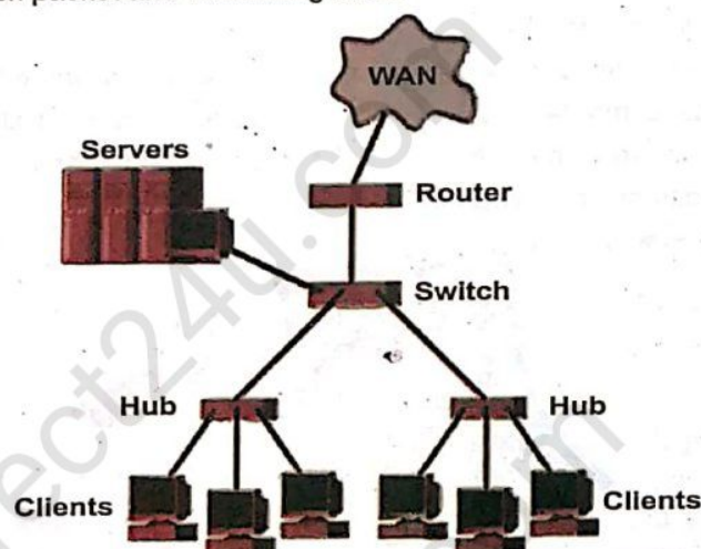
Figure 5.15 Communication Devices
