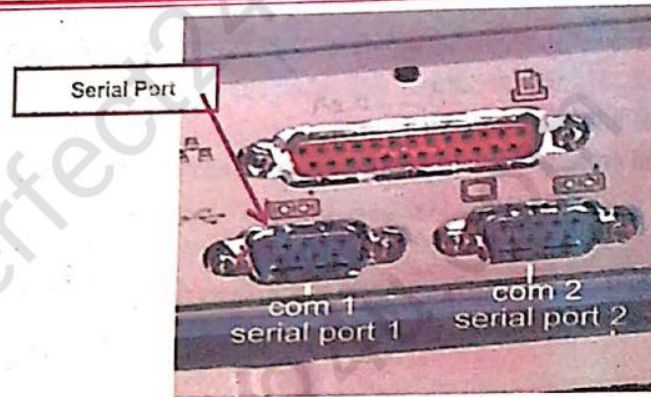
Figure 4.13 Serial Ports
