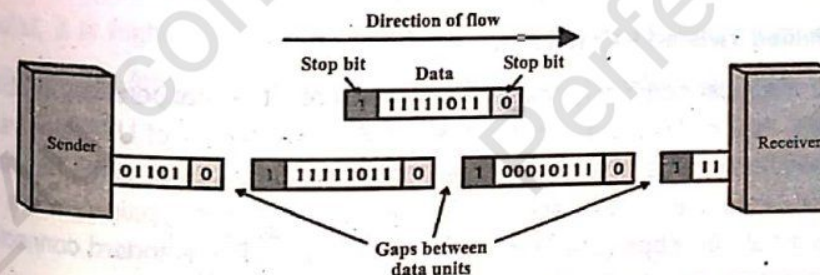
Figure 5.7 Asynchronous Transmission
