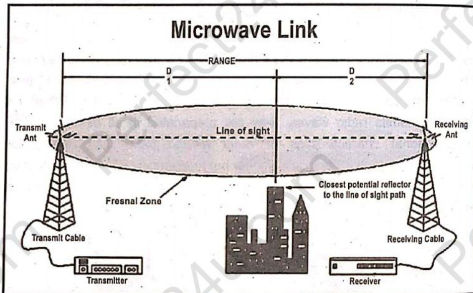
Figure 5.12 Microwave transmission
