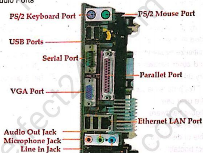
Figure 4.6 Ports
