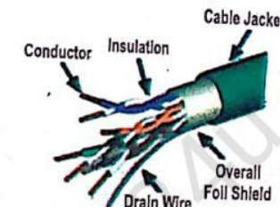
Figure 5.8 (b) Shielded Twisted Pair Cable
