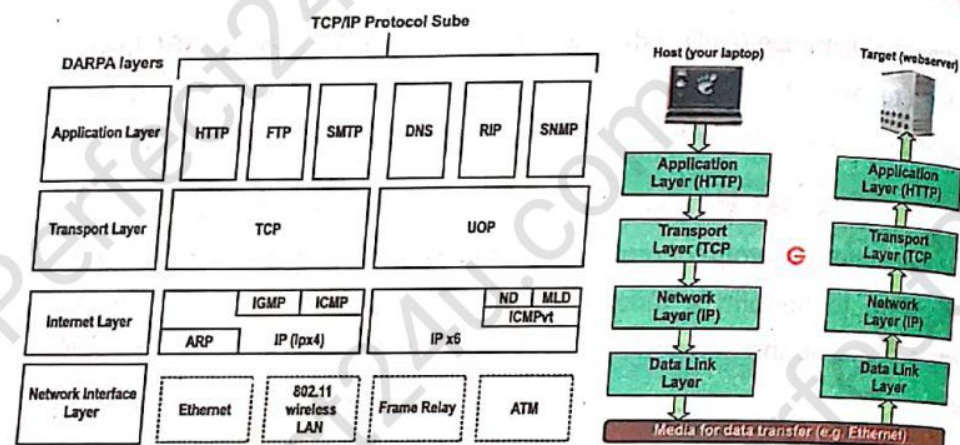
Figure 5.28 The architecture of the TCP/IP protocol suite
