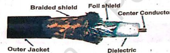
Figure 5.9 Coaxial Cable
