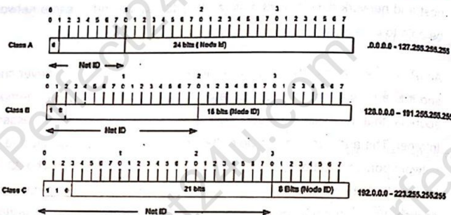
Figure 5.30 Classes of IP Addresses
