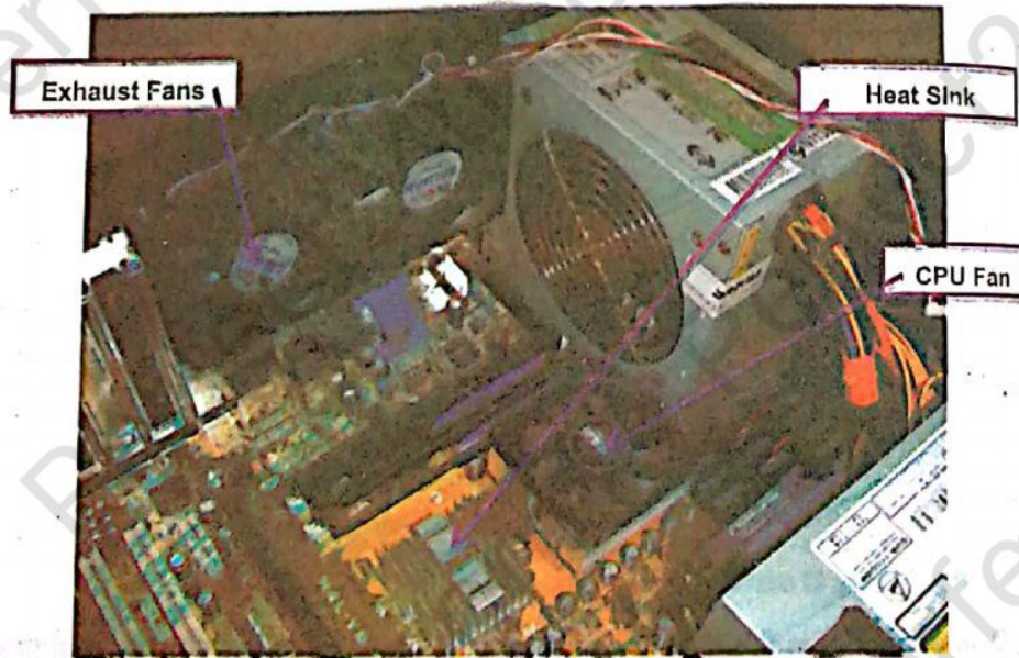
Figure 4.12 Cooling System
