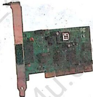
Figure 4.20 MODEM Card
