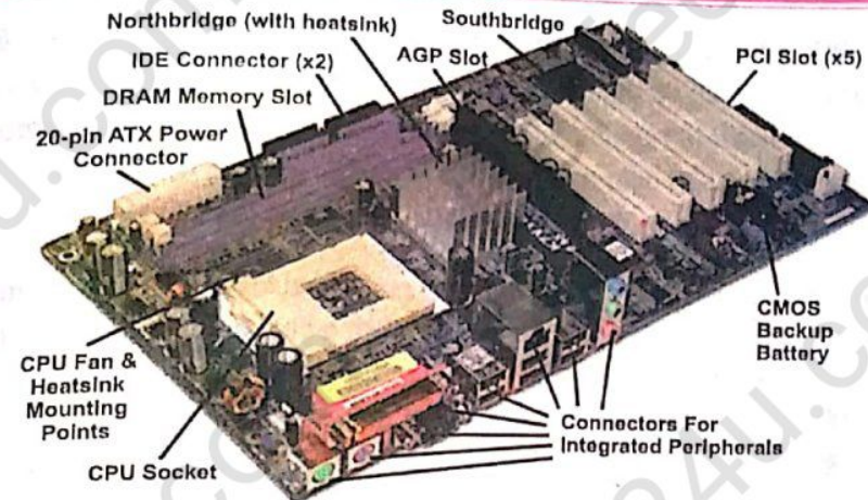
Figure 4.5 A Motherboard
