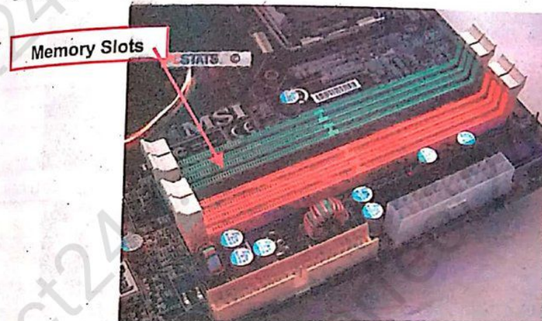
Figure 4.11 Memory Slots
