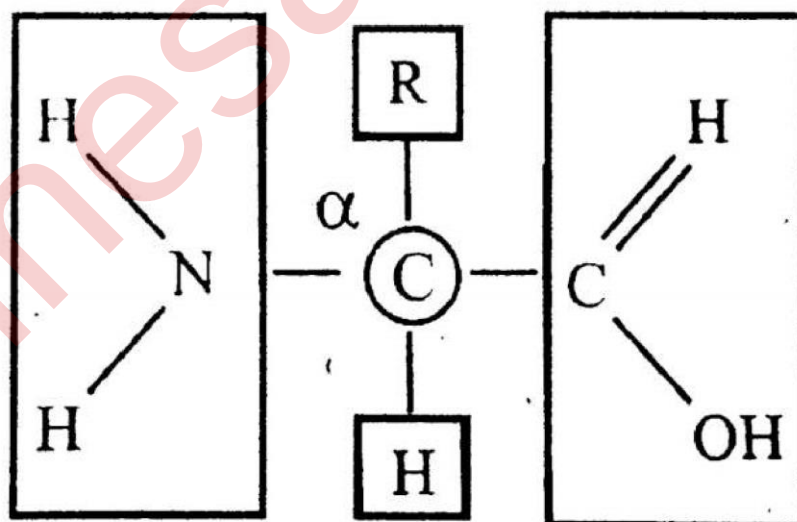
General structure of an amino acid
