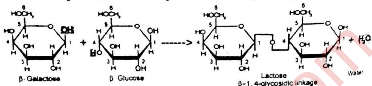
Formation of lactose
