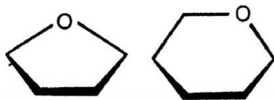
Furanose ring Pyranose ring
