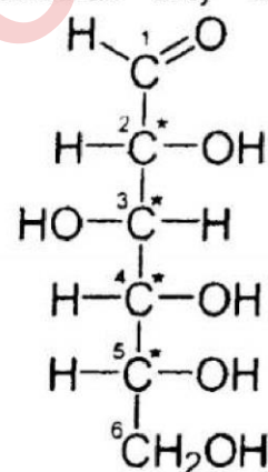
Glucose: asymmetric carbon are shown by sterics
