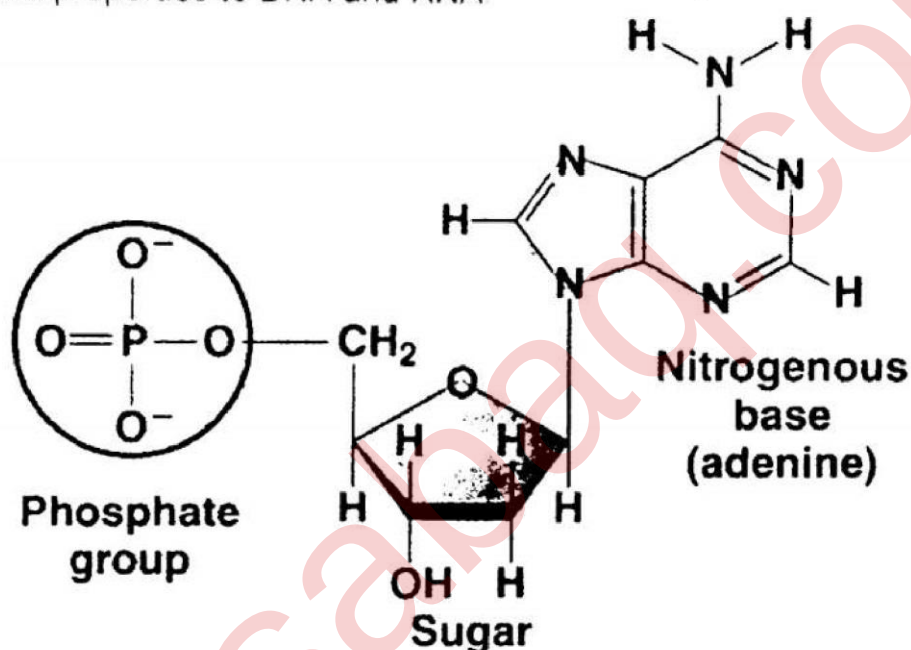
Structure of a nucleotide
