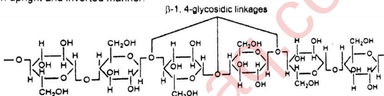
Structure of cellulose
