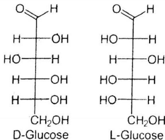
An example of enantiomers
