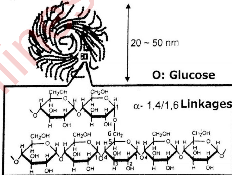
Glycogen (Highly branched unlike amylopectin)
