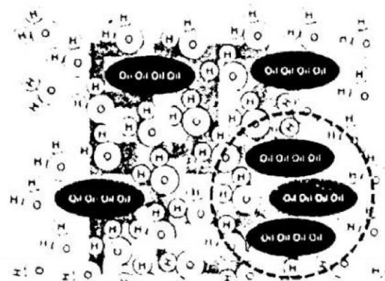
Hydrophobic exclusion
