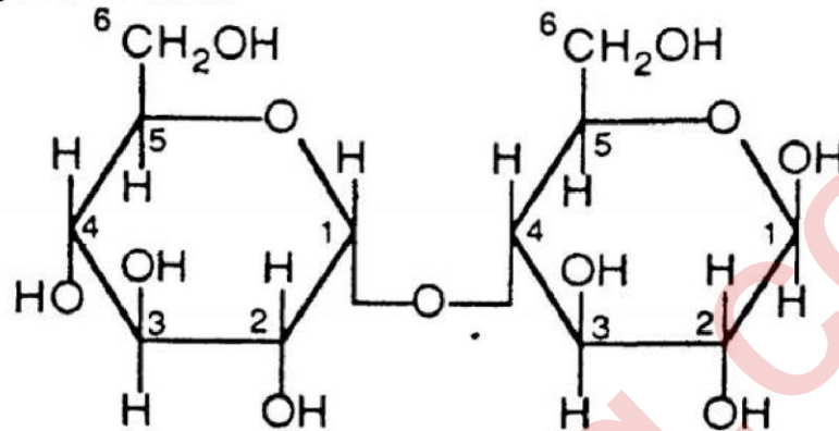
Maltose
