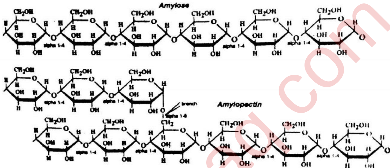
Structure of starches
