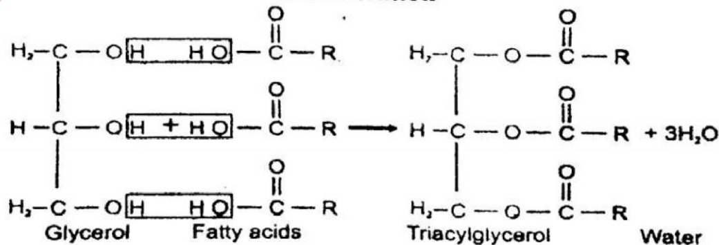
Formation of a triacylglycerol (neutral lipid)
