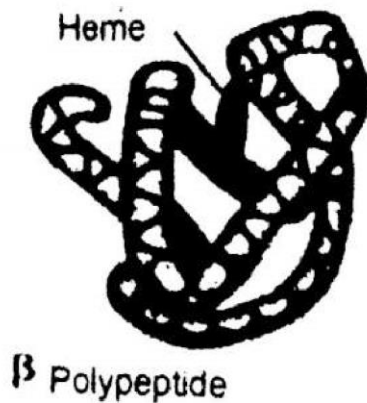
(c) Tertiary structure
