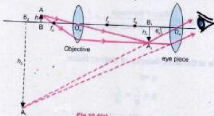
Fig. 10.4 (a). Ray diagram of a Compound Microscope
