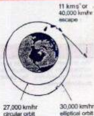
Satellites Orbits
