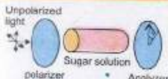
Sugar solution rotates the plane of polarization of incident light so that it is no longer horizontal but at an angle. The analyzer thus stops the light when rotated from the vertical (crossed) position.
