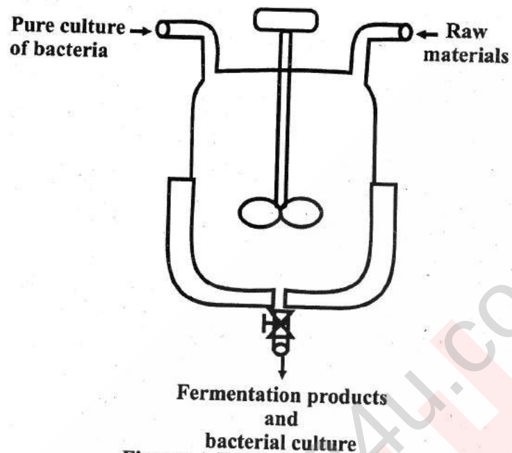
Figure: A Batch Fermenter
