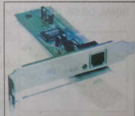
Fig.4.18 10/100 Ethernet Card
