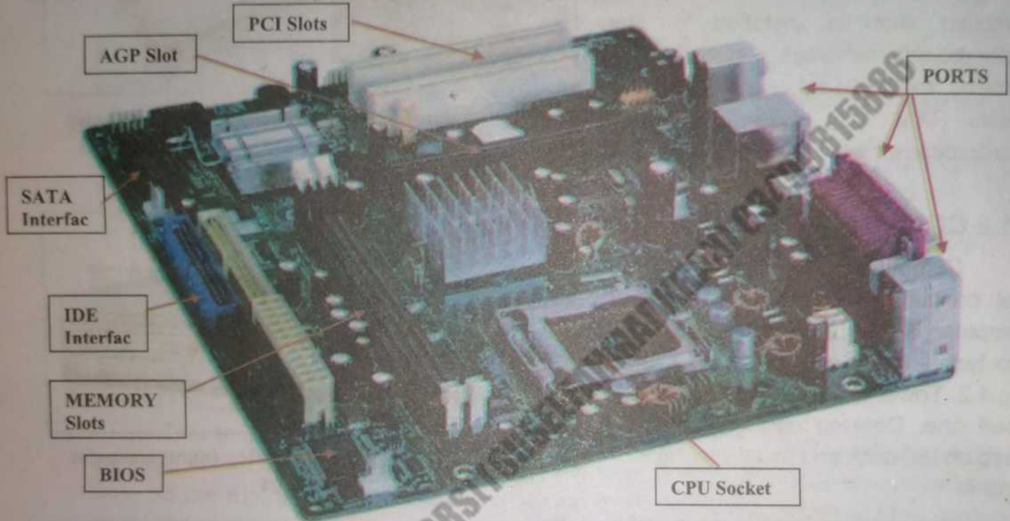
Fig.4.4 Motherboard
