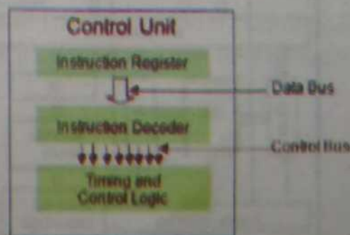
Fig.3.3 Control Unit
