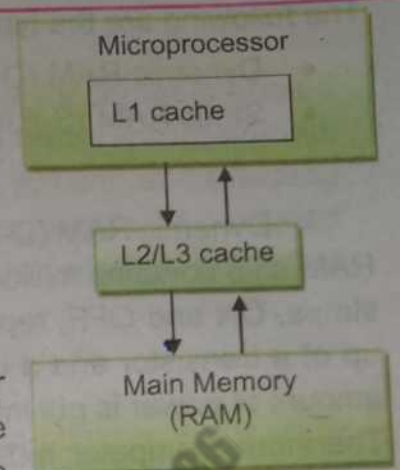
Fig.2.6 L1, L2 and L3 Cache Memory
