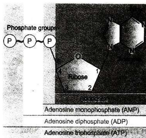
(Figure 7.3) Molecular structure of Adenosine Triphosphate (ATP)
